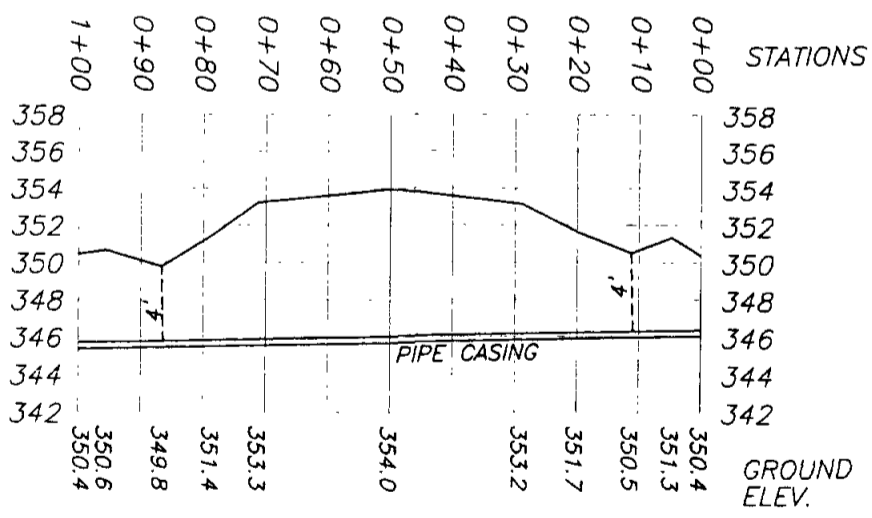
ELEVATION VIEW OF PROPOSED 3" PIPELINE CROSSING HIGHWAY
